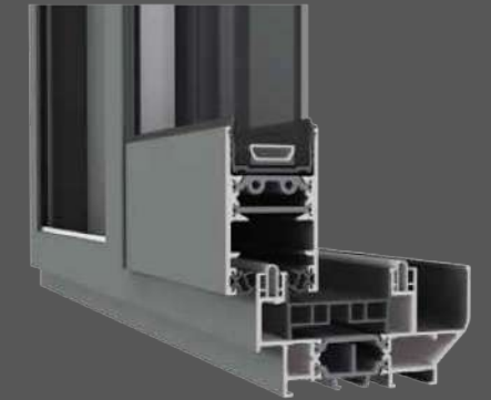
REYNAERS CONCEPTPATIO 68 PA (CP68 PA)
